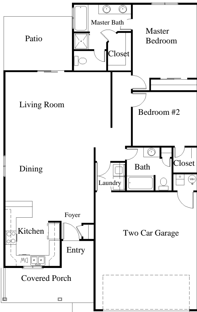
Main Floor Slab Version
