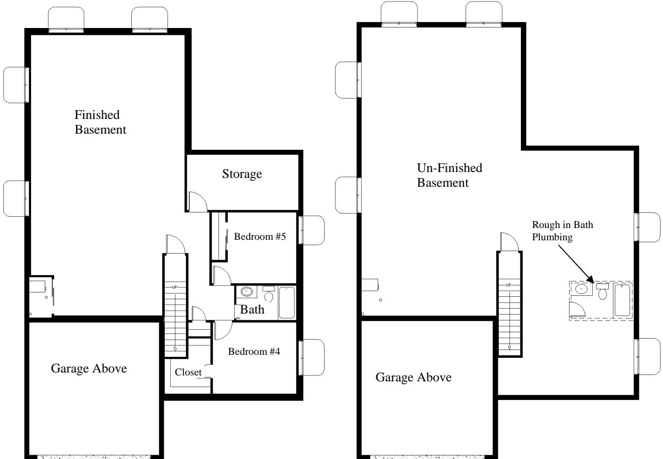
Finished Basement (option)
