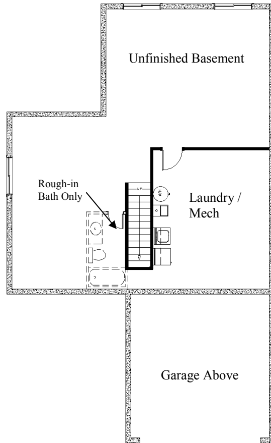
Unfinished Basement
